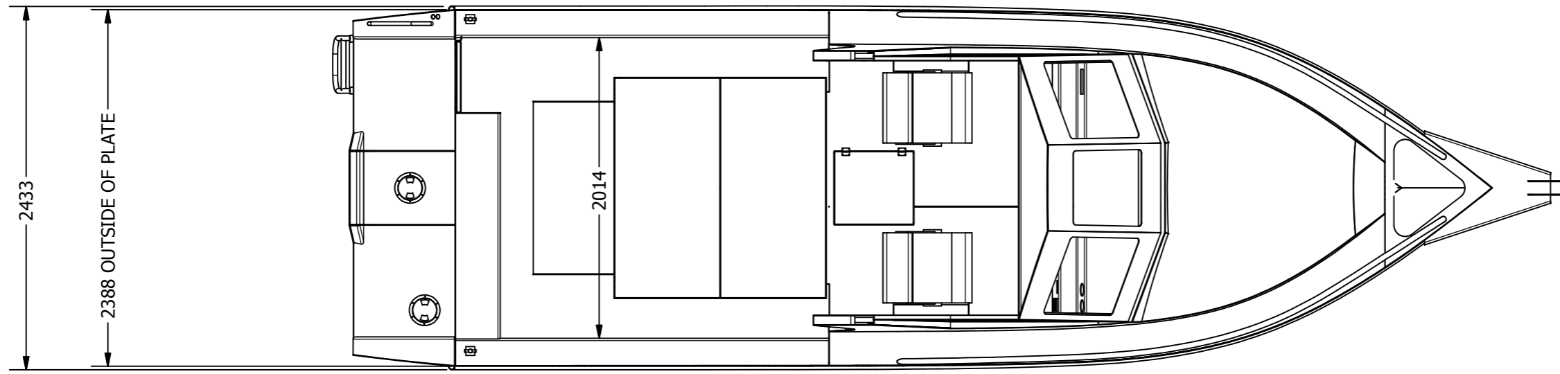
PLAN SCALE 1:35 (ROOF REMOVED)
