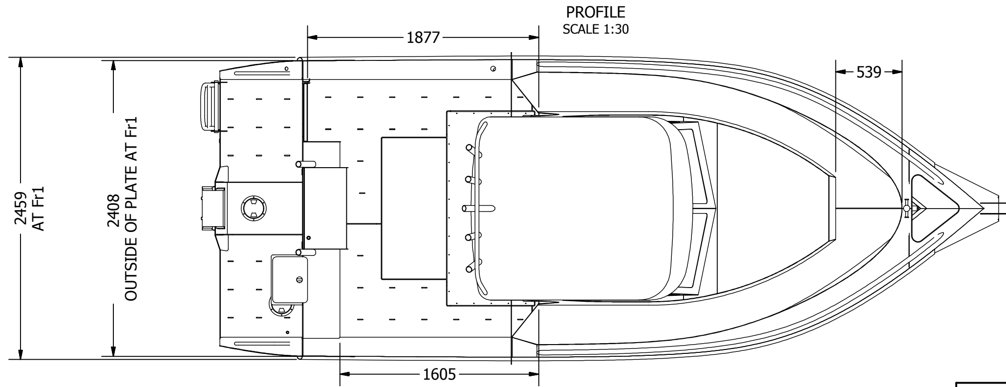
PLAN SCALE 1:30
