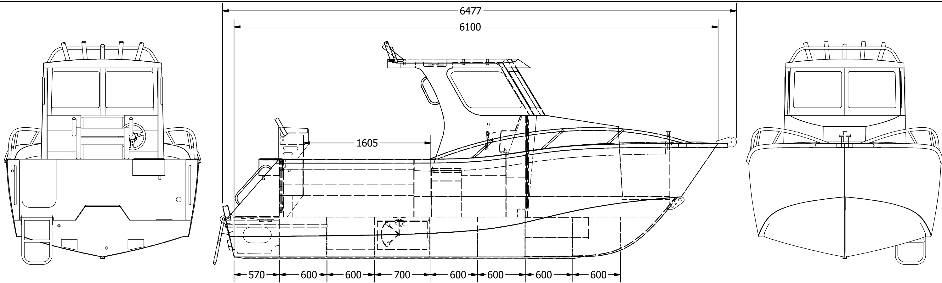
PROFILE SCALE 1:30
