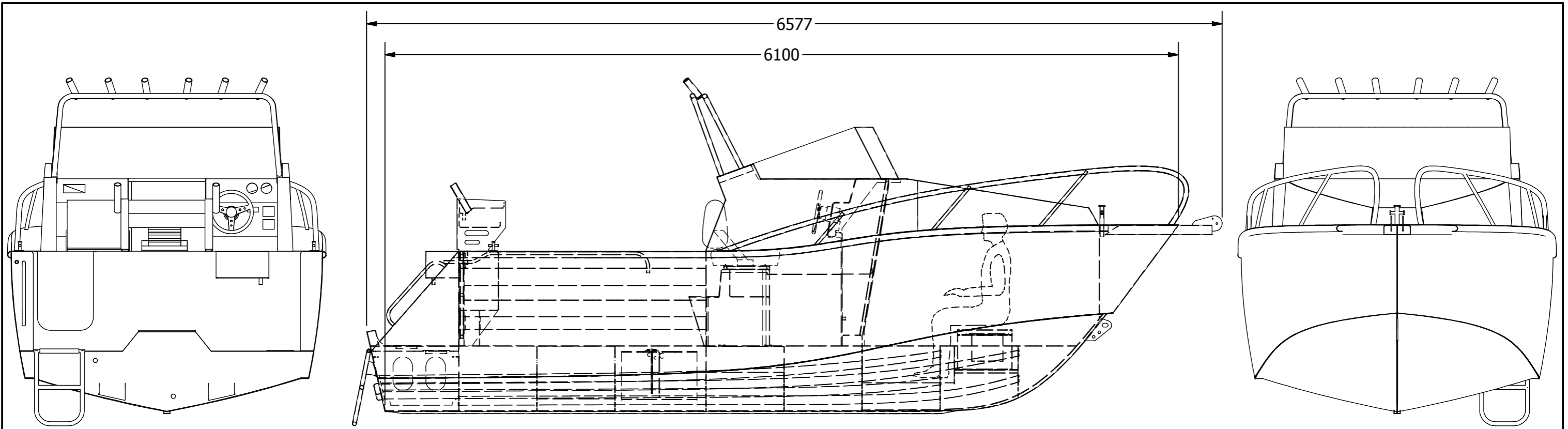
PROFILE SCALE 1:30
