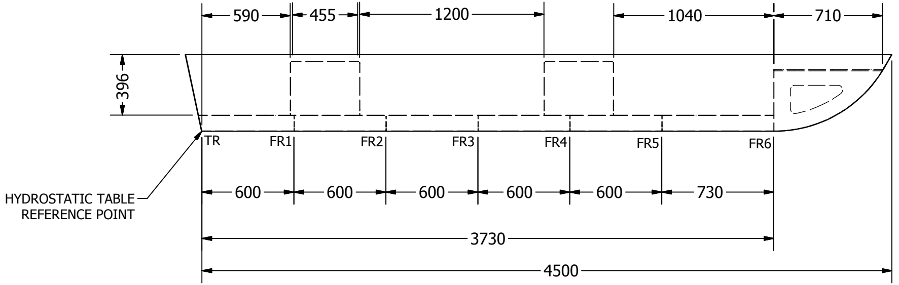
PROFILE VIEW (FENDER NOT SHOWN) SCALE 1:25
